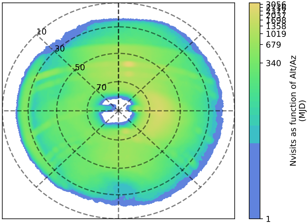
ddf_acor_sf10_lsf30_lsr10_v3.4_10yrs r: Nvisits as function of Alt/Az
