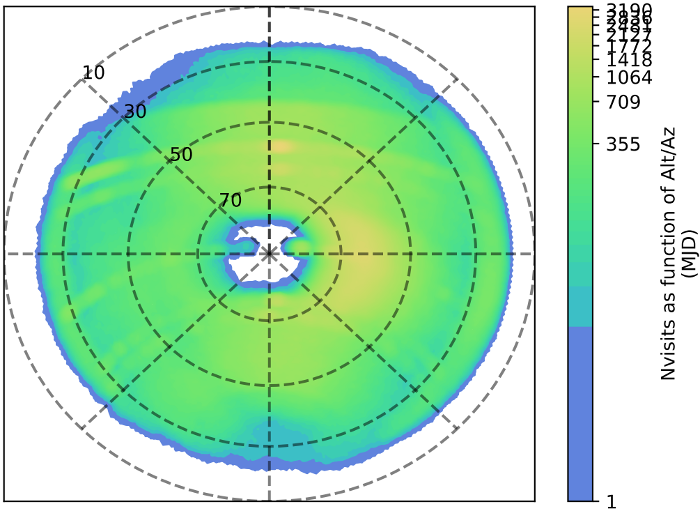
ddf_acor_sf10_ls30_lsr10_v3.4_10yrs i: Nvisits as function of Alt/Az
