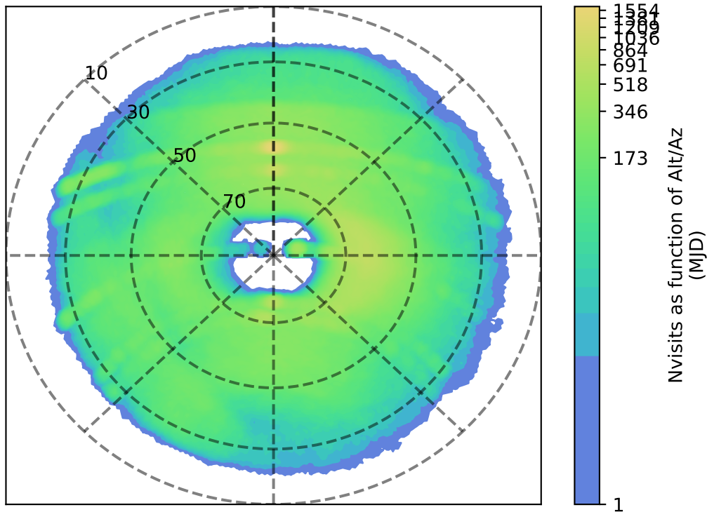
ddf_acor_sf10_lsf30_lsr10_v3.4_10yrs g: Nvisits as function of Alt/Az
