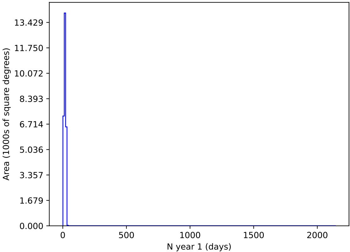
ddf_acor_sf10_lsf30_lsr10_v3.4_10yrs i and night < 365: N year 1
