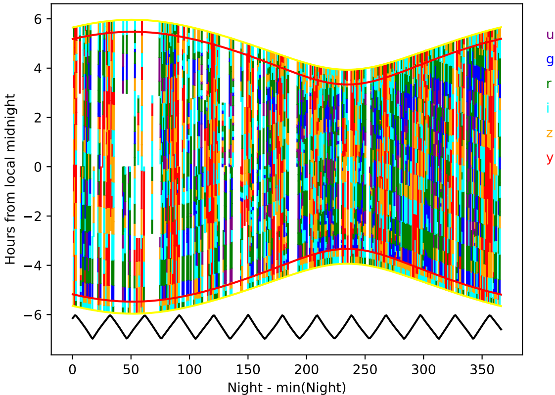
ddf_acor_sf10_lsf30_lsr10_v3.4_10yrs year 9-10: Hourglass
