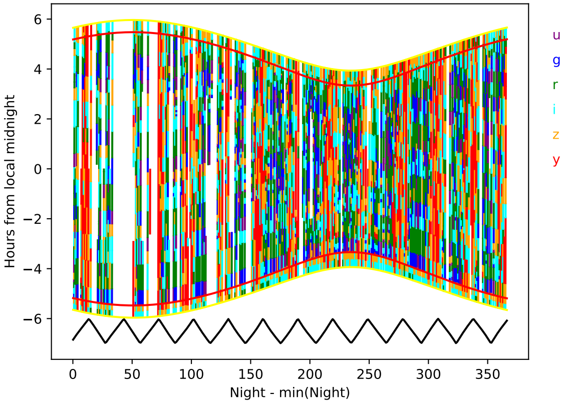
ddf_acor_sf10_lsf30_lsr10_v3.4_10yrs year 8-9: Hourglass
