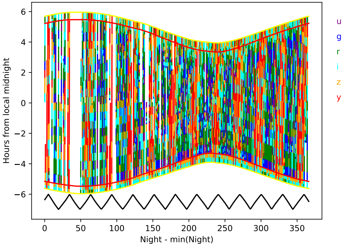
ddf_acor_sf10_lsf30_lsr10_v3.4_10yrs year 6-7: Hourglass
