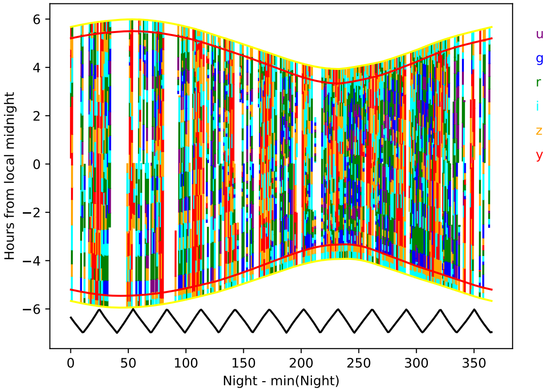
ddf_acor_sf10_lsf30_lsr10_v3.4_10yrs year 4-5: Hourglass
