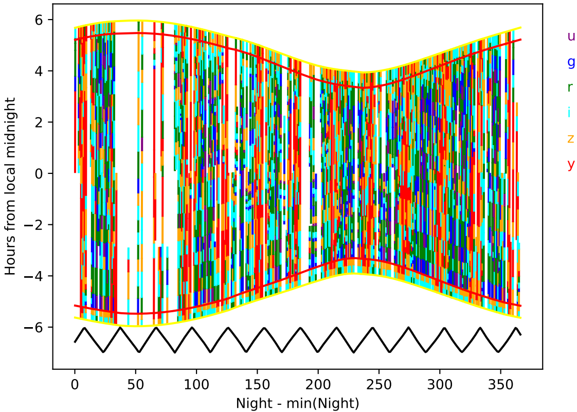
ddf_acor_sf10_lsf30_lsr10_v3.4_10yrs year 3-4: Hourglass
