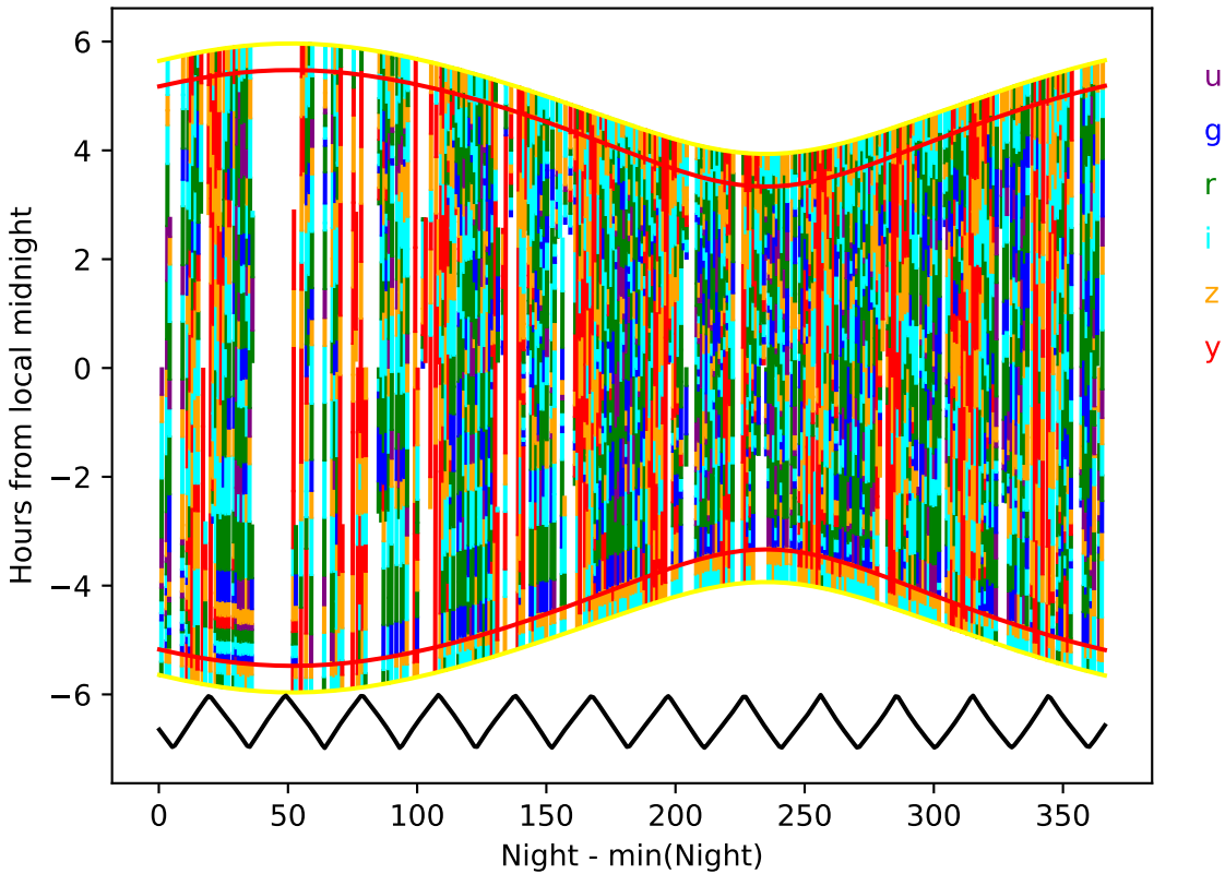
ddf_acor_sf10_lsf30_lsr10_v3.4_10yrs year 2-3: Hourglass
