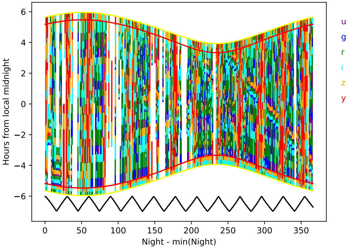
ddf_acor_sf10_lsf30_lsr10_v3.4_10yrs year 1-2: Hourglass
