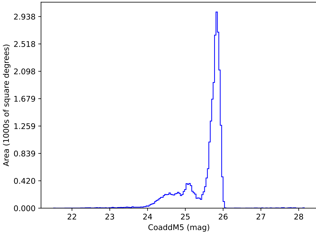
ddf_acor_sf10_lsf30_lsr10_v3.4_10yrs z: CoaddM5
