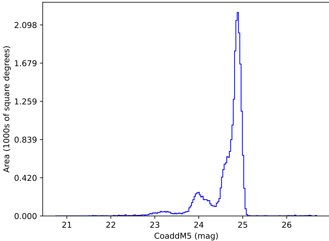
ddf_acor_sf10_lsf30_lsr10_v3.4_10yrs y: CoaddM5
