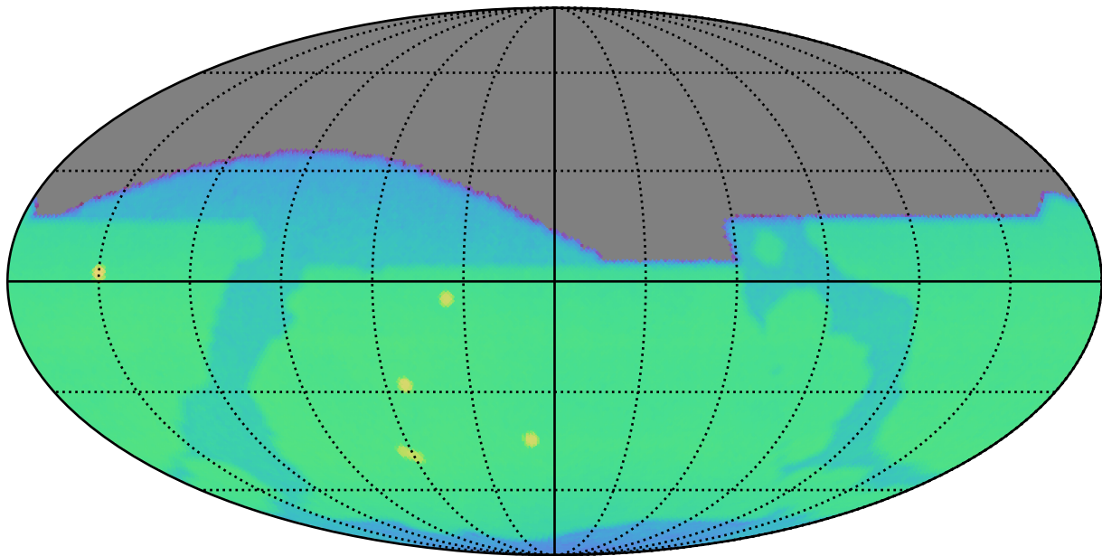
ddf_acor_sf10_lsf30_lsr10_v3.4_10yrs i: CoaddM5
