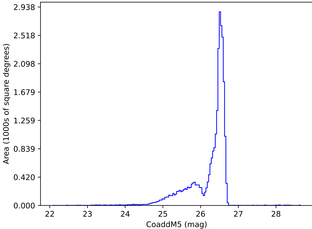
ddf_acor_sf10_lsf30_lsr10_v3.4_10yrs i: CoaddM5
