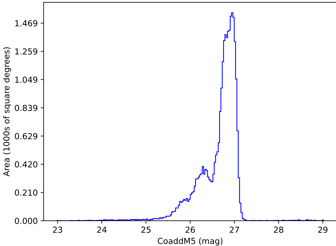
ddf_acor_sf10_lsf30_lsr10_v3.4_10yrs g: CoaddM5
