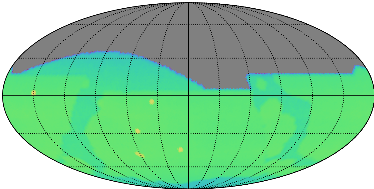
ddf_acor_sf10_lsf30_lsr10_v3.4_10yrs : CoaddM5
