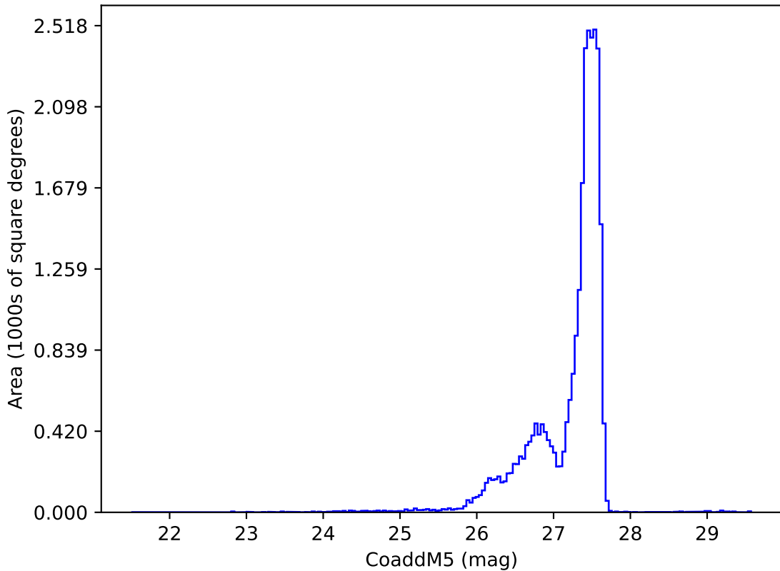
ddf_acor_sf10_lsf30_lsr10_v3.4_10yrs : CoaddM5
