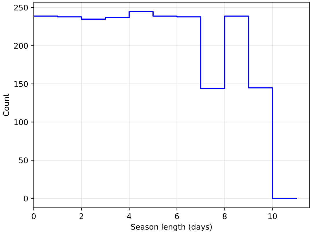
ddf_acor_sf10_lsf30_lsr10_v3.4_10yrs DD:ECDFS all bands: SeasonLength
