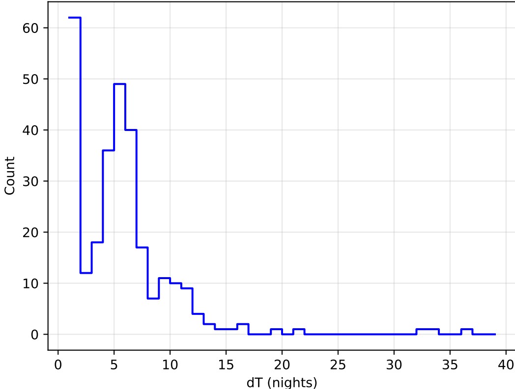
ddf_acor_sf10_lsf30_lsr10_v3.4_10yrs all bands: DD:XMM_LSS Delta Nights Histogram
