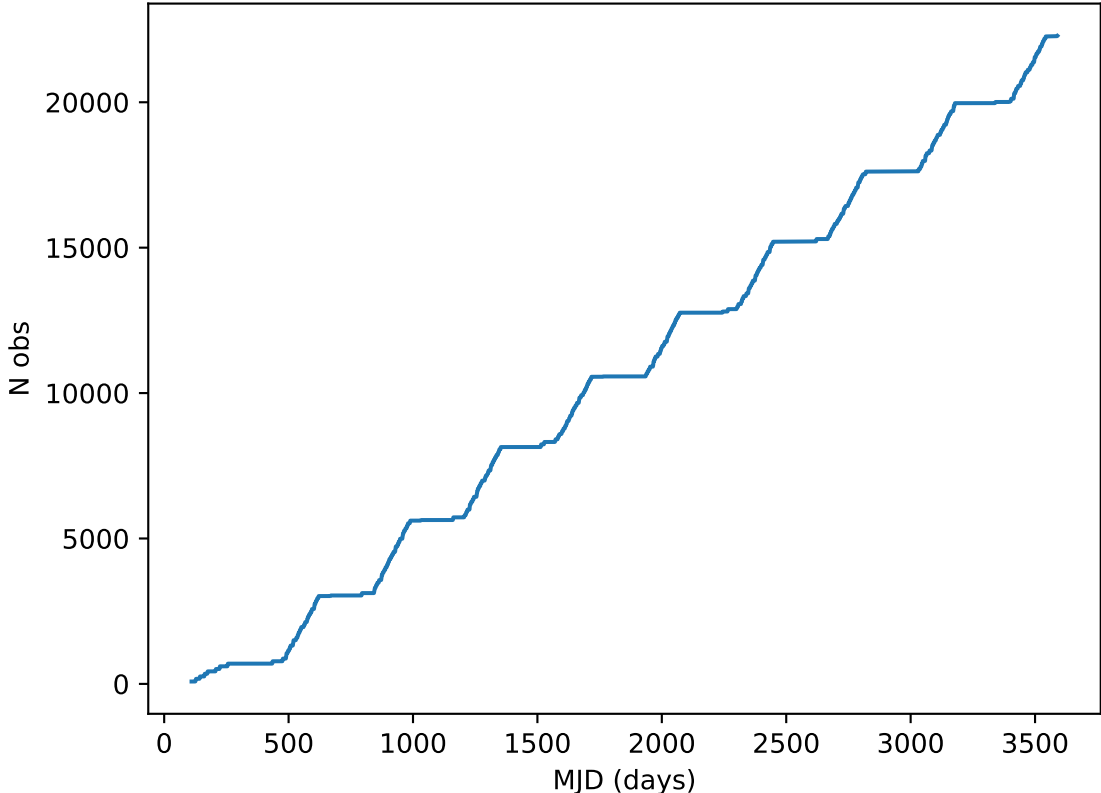
ddf_acor_sf10_lsf30_lsr10_v3.4_10yrs all bands: DD:XMM_LSS Cumulative NVisits
