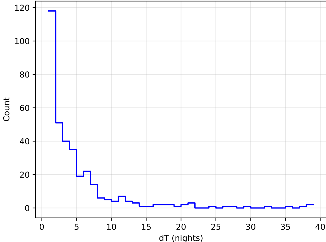
ddf_acor_sf10_lsf30_lsr10_v3.4_10yrs all bands: DD:WFD Delta Nights Histogram
