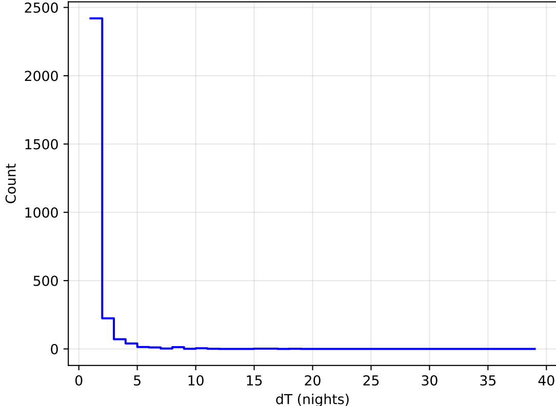
ddf_acor_sf10_lsf30_lsr10_v3.4_10yrs all bands: DD:WFD Delta Nights Histogram
