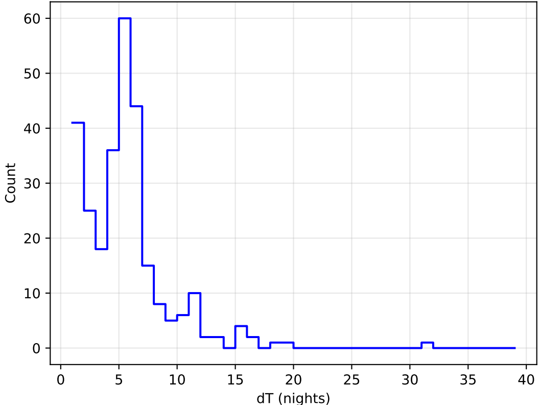
ddf_acor_sf10_lsf30_lsr10_v3.4_10yrs all bands: DD:ELAISS1 Delta Nights Histogram
