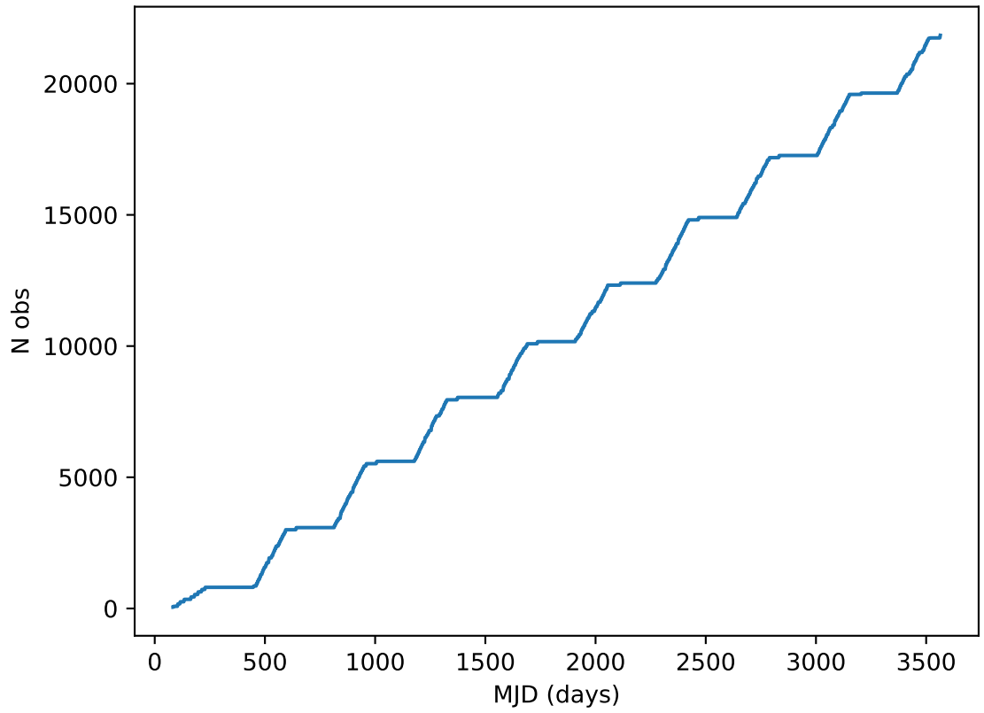
ddf_acor_sf10_lsf30_lsr10_v3.4_10yrs all bands: DD:ELAISS1 Cumulative NVisits
