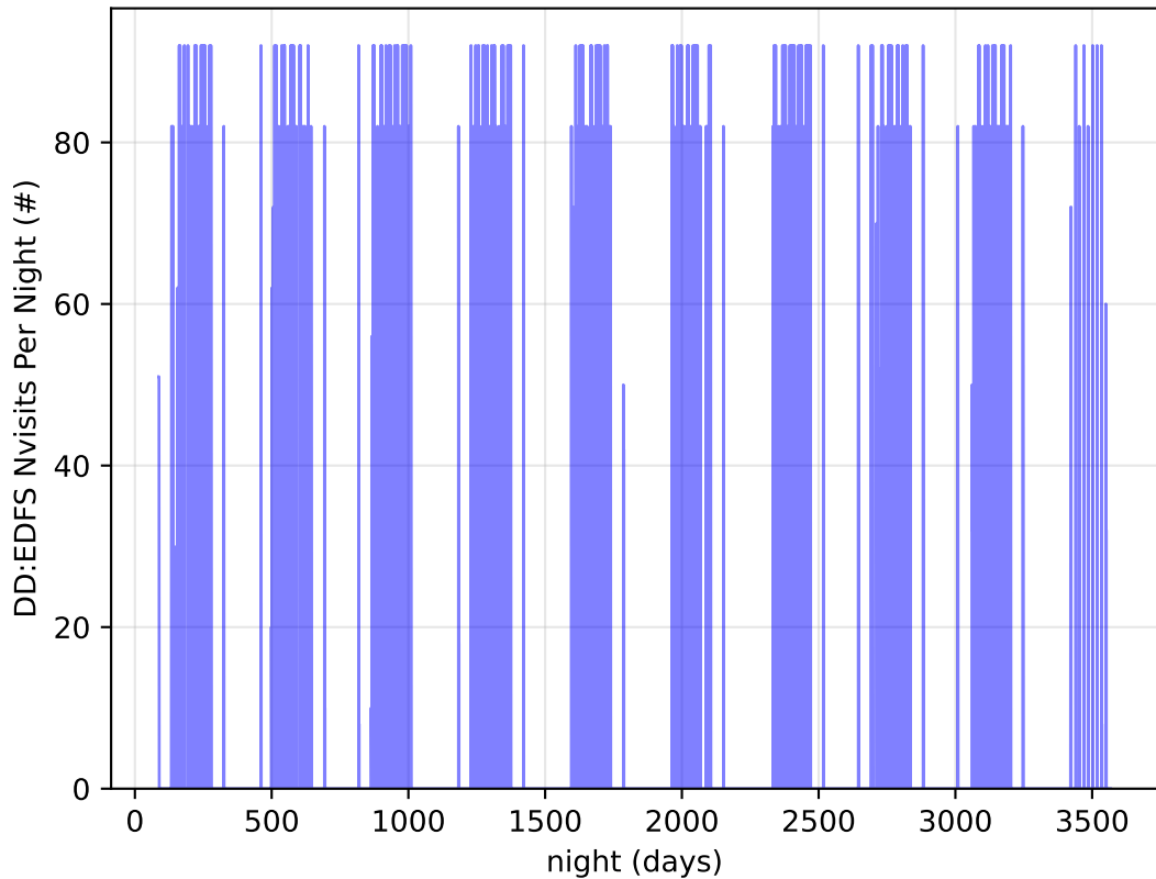
ddf_acor_sf10_lsf30_lsr10_v3.4_10yrs all bands: DD:EDFS Nvisits Per Night
