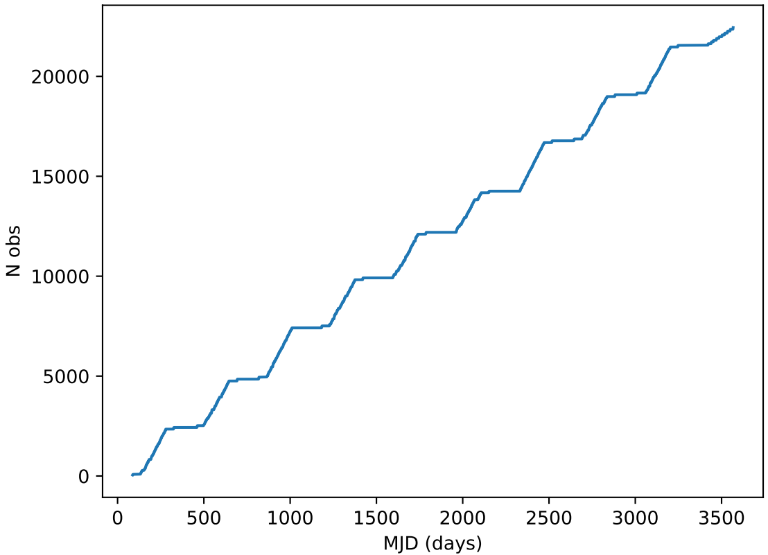
ddf_acor_sf10_lsf30_lsr10_v3.4_10yrs all bands: DD:EDFS Cumulative NVisits
