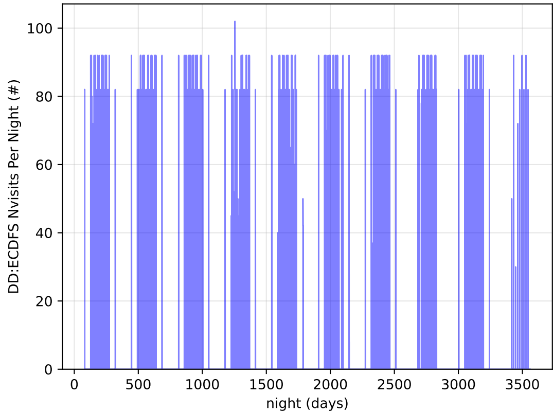
ddf_acor_sf10_lsf30_lsr10_v3.4_10yrs all bands: DD:ECDFS Nvisits Per Night
