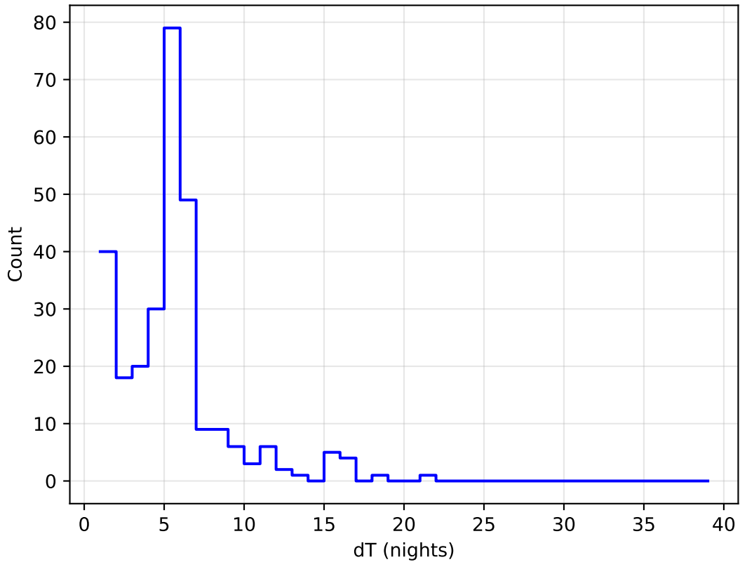
ddf_acor_sf10_lsf30_lsr10_v3.4_10yrs all bands: DD:ECDFS Delta Nights Histogram
