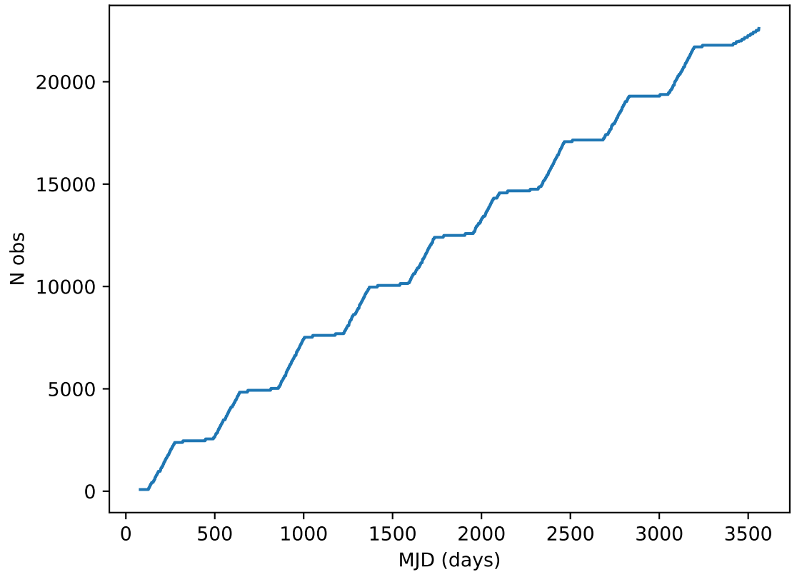
ddf_acor_sf10_lsf30_lsr10_v3.4_10yrs all bands: DD:ECDFS Cumulative NVisits
