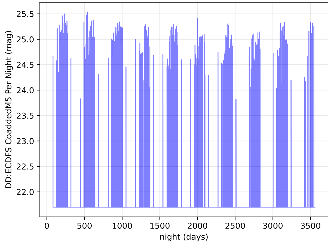
ddf_acor_sf10_lsf30_lsr10_v3.4_10yrs z band: DD:ECDFS CoaddedM5 Per Night
