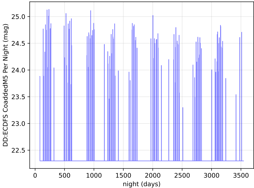
ddf_acor_sf10_lsf30_lsr10_v3.4_10yrs u band: DD:ECDFS CoaddedM5 Per Night
