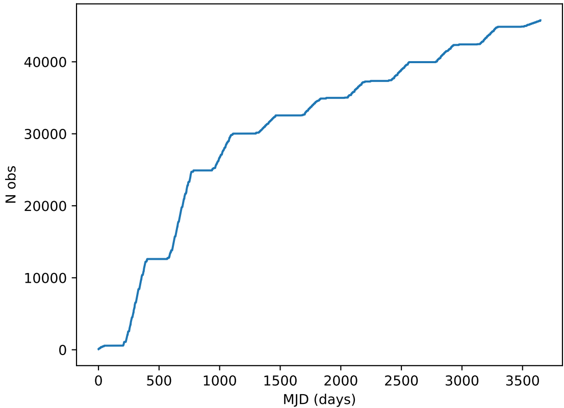
ddf_acor_sf10_lsf30_lsr10_v3.4_10yrs all bands: DD: COSMOS Cumulative NVisits
