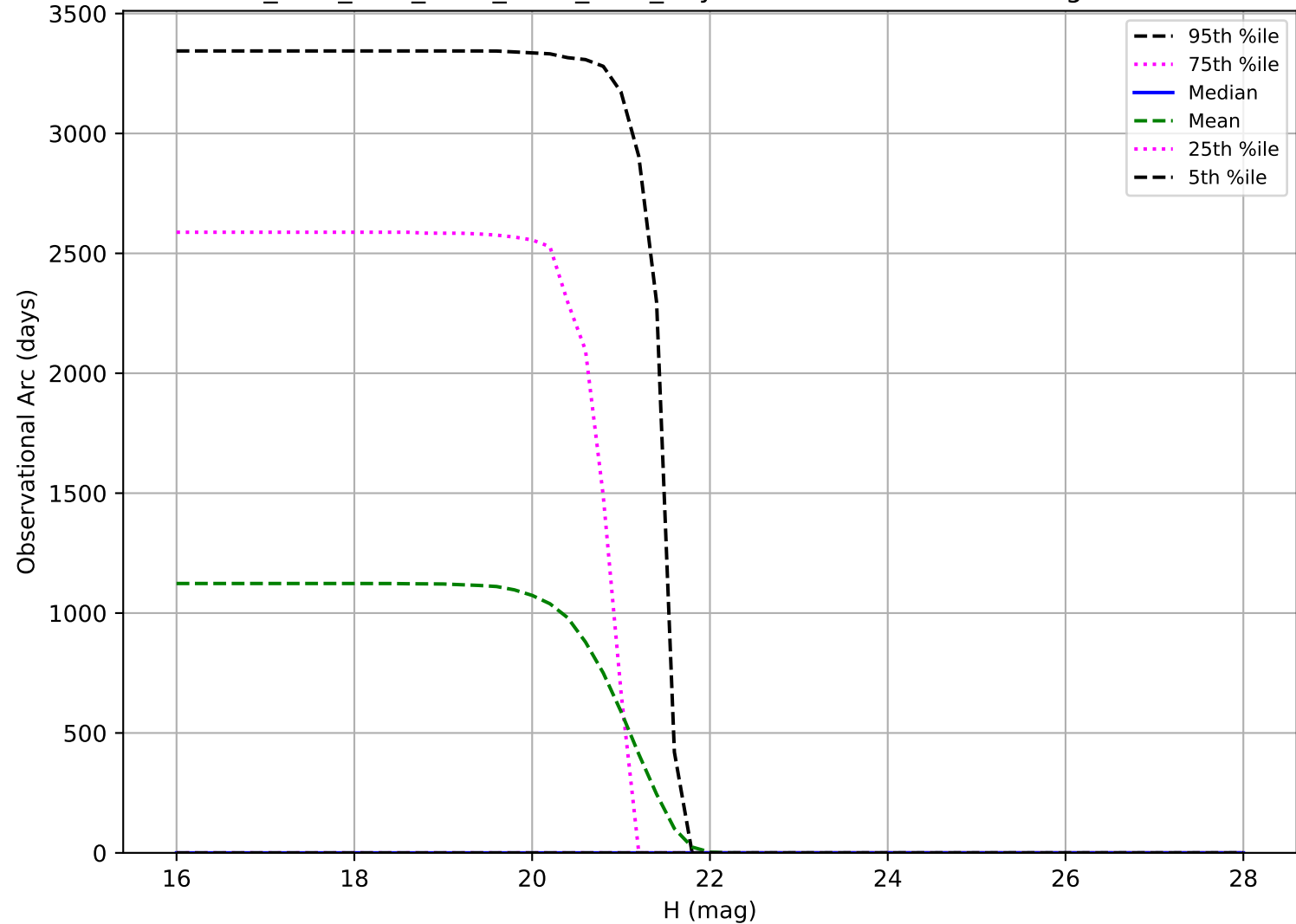
ddf_acor_sf10_lsf20_lsr50_v3.4_10yrs: Observational Arc Length Vatira
