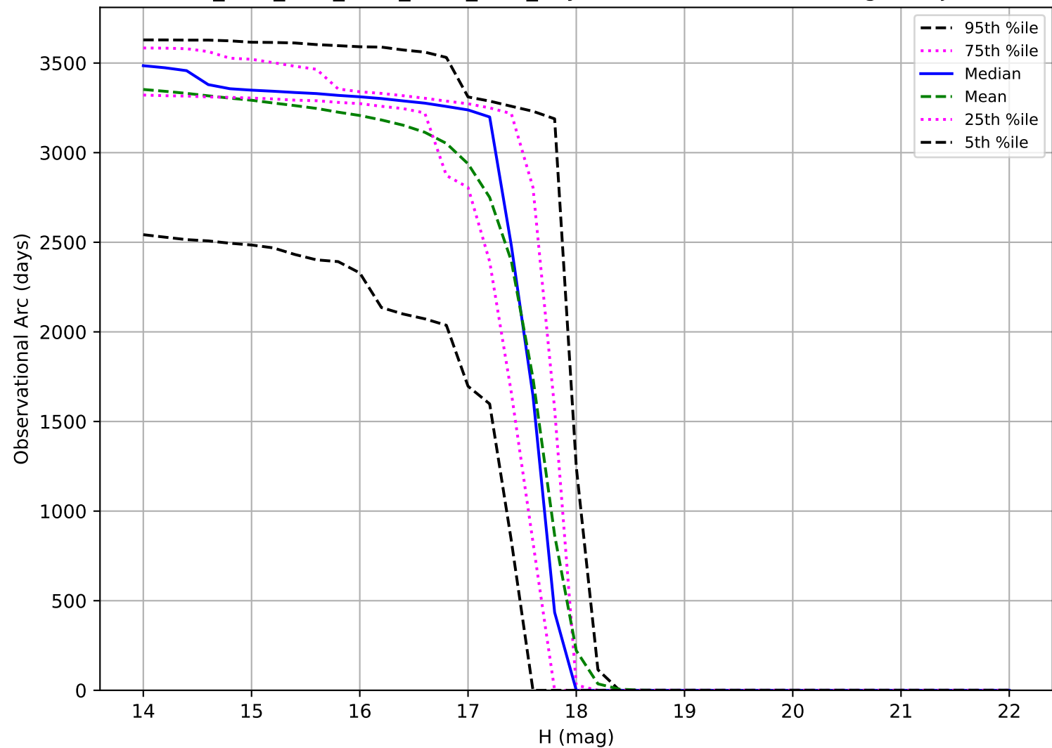
ddf_acor_sf10_lsf20_lsr50_v3.4_10yrs: Observational Arc Length Trojan
