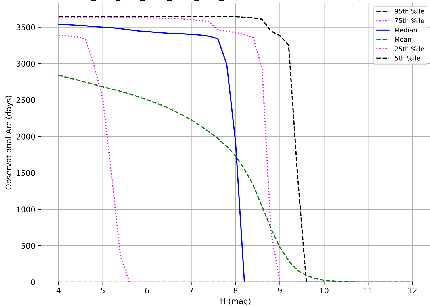
ddf_acor_sf10_Isf20_Isr50_v3.4_10yrs: Observational Arc Length TNO
