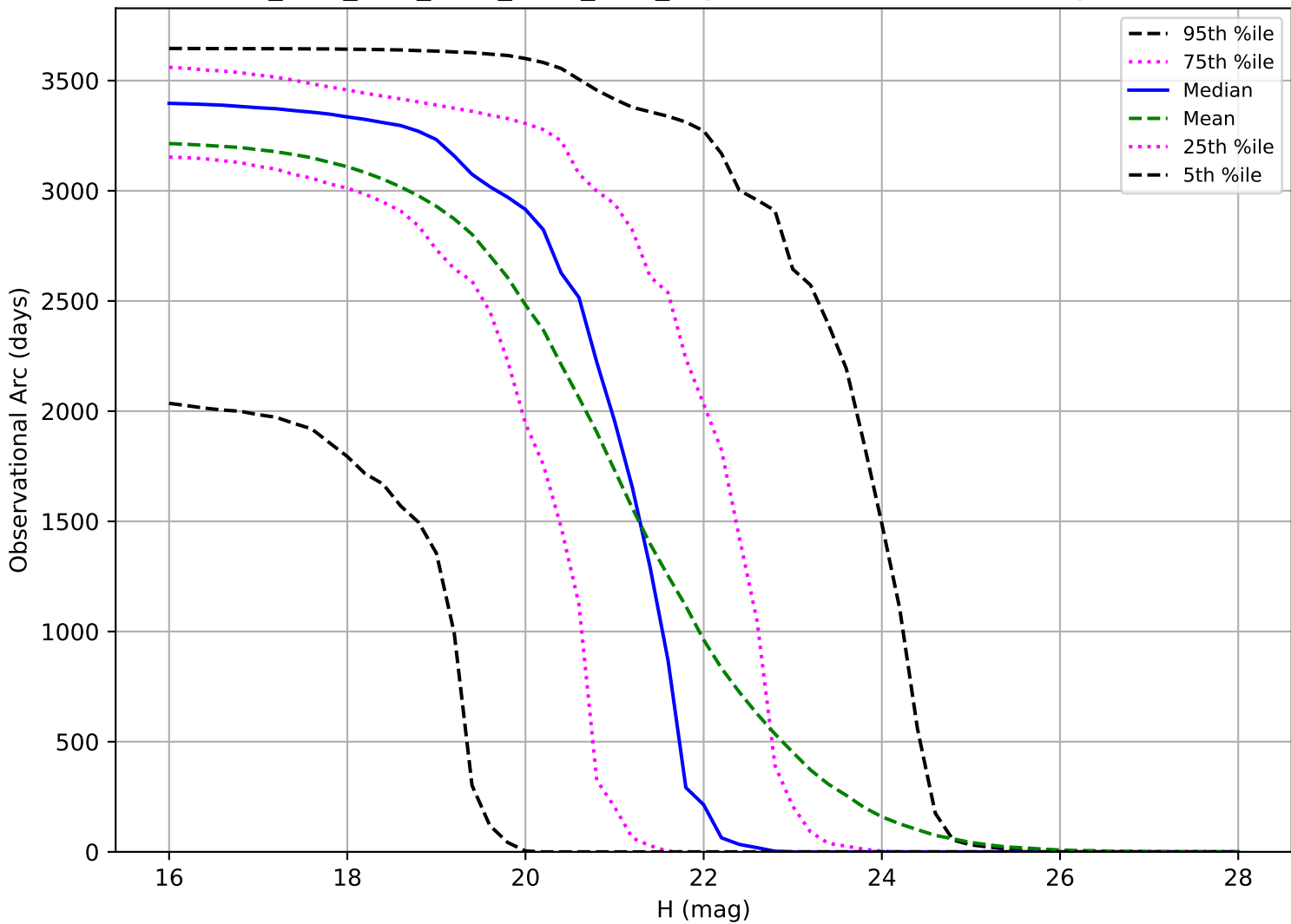
ddf_acor_sf10_lsf20_lsr50_v3.4_10yrs: Observational Arc Length PHA
