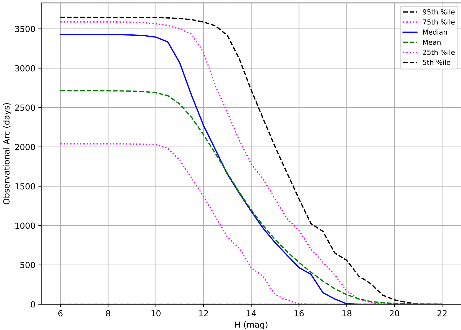
ddf_acor_sf10_lsf20_lsr50_v3.4_10yrs: Observational Arc Length OCC_r5
