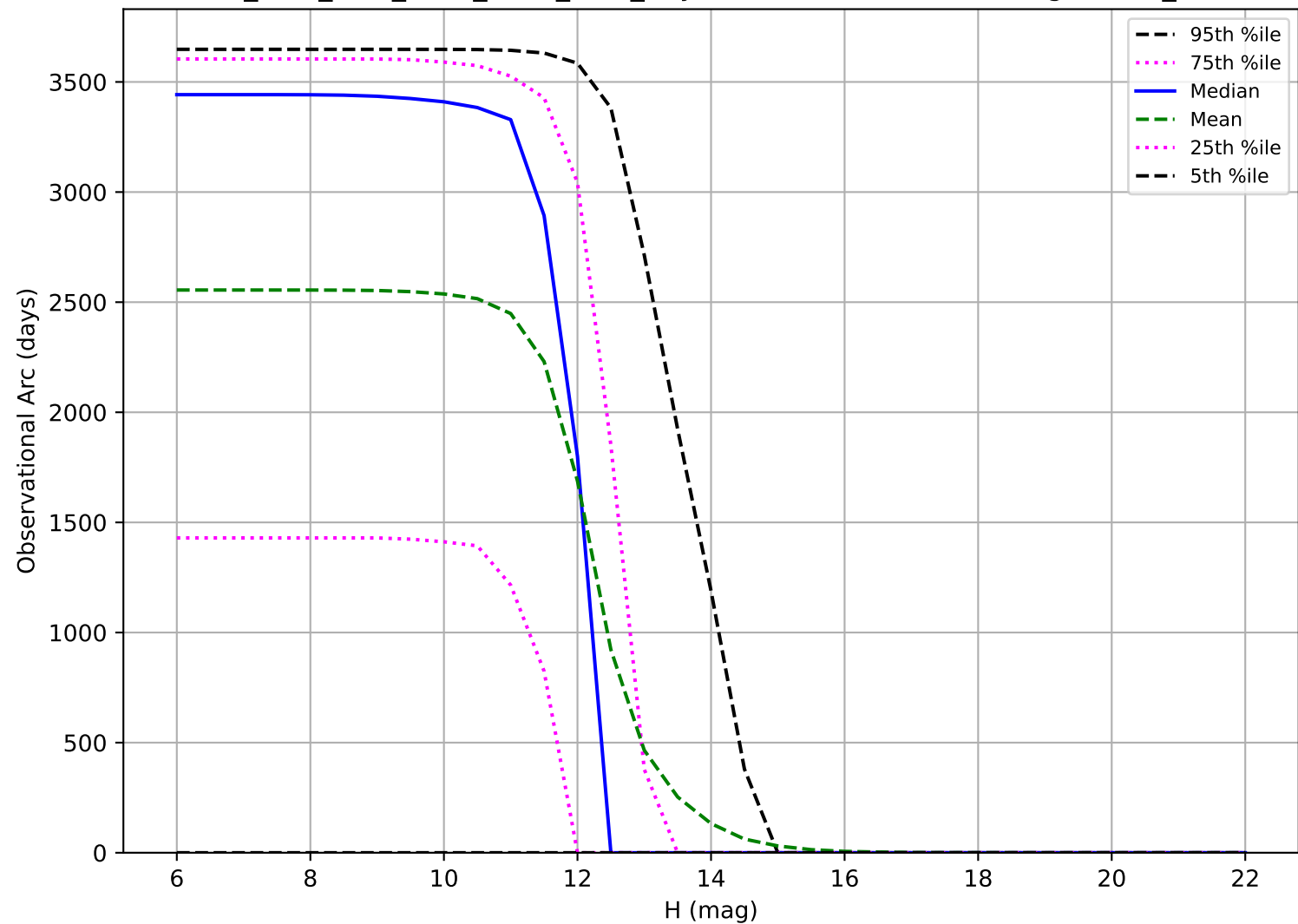
ddf_acor_sf10_lsf20_lsr50_v3.4_10yrs: Observational Arc Length OCC_r20
