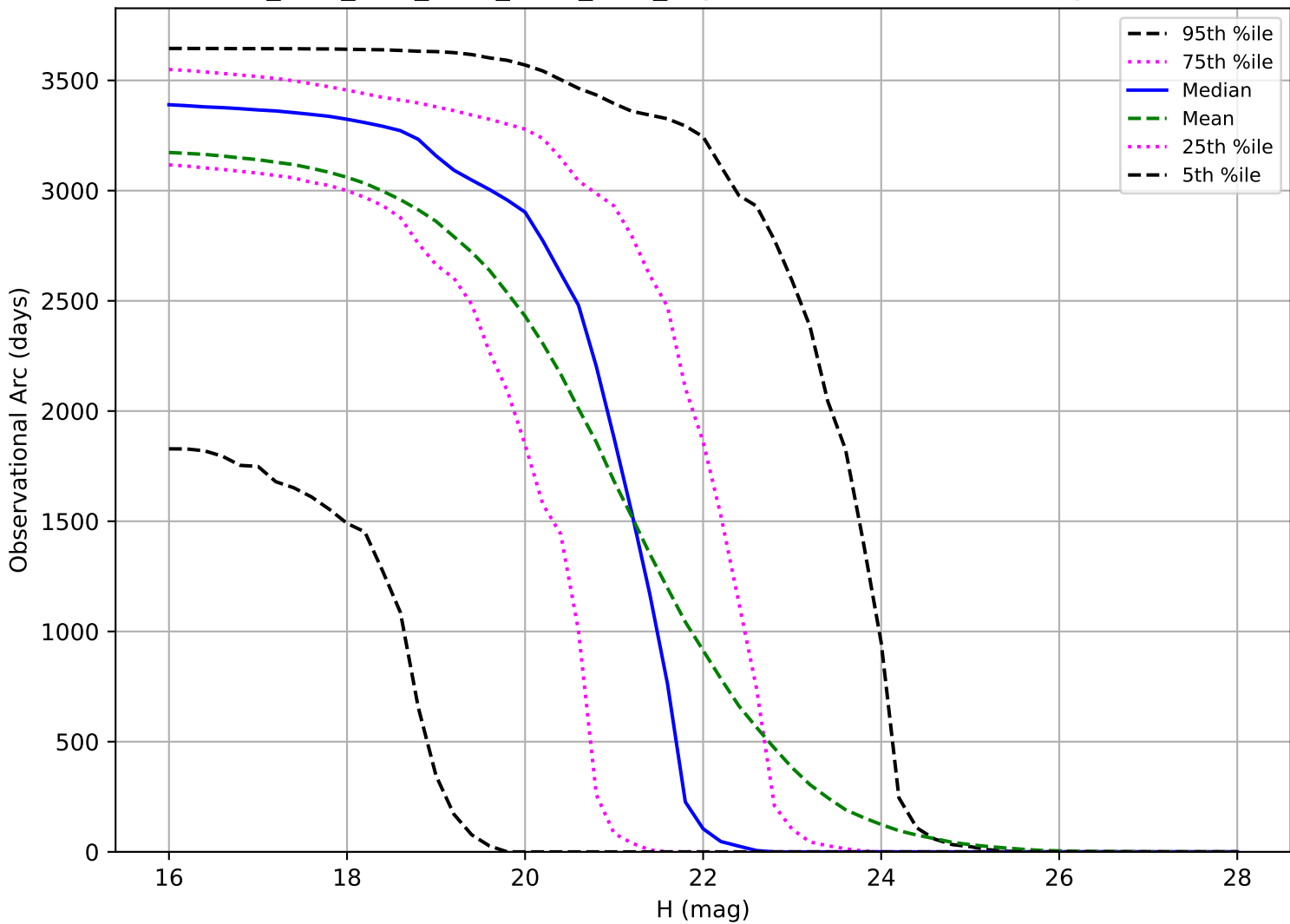
ddf_acor_sf10_lsf20_lsr50_v3.4_10yrs: Observational Arc Length NEO
