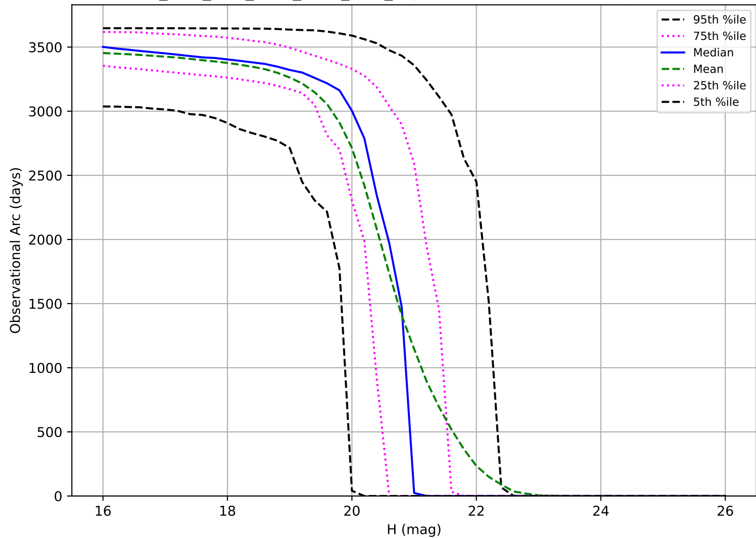
ddf_acor_sf10_lsf20_lsr50_v3.4_10yrs: Observational Arc Length MBA
