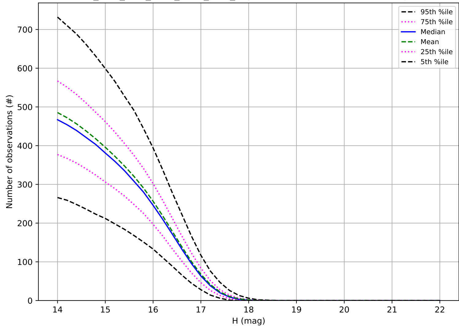
ddf_acor_sf10_lsf20_lsr50_v3.4_10yrs: Number of observations Trojan
