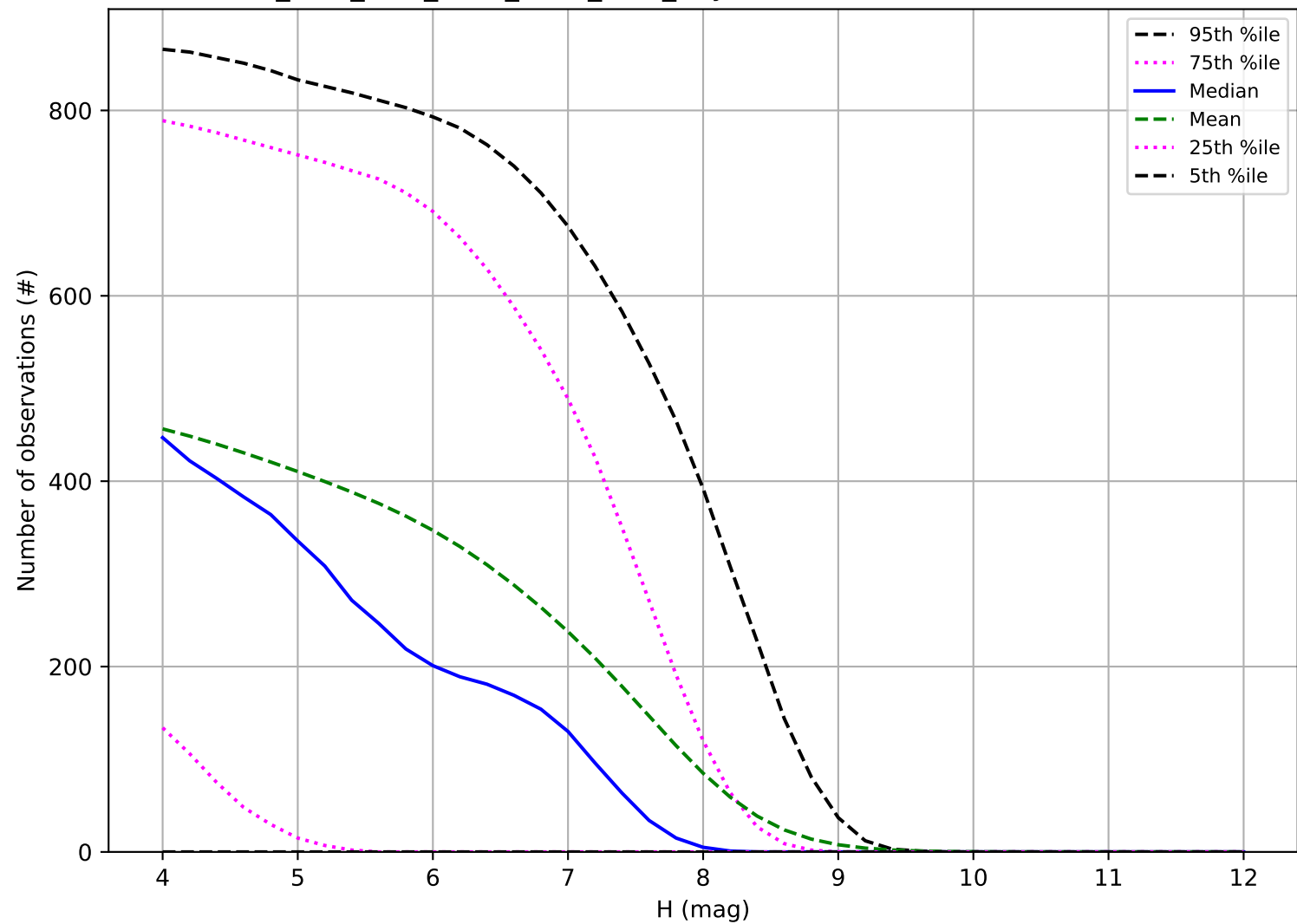
ddf_acor_sf10_lsf20_lsr50_v3.4_10yrs: Number of observations TNO
