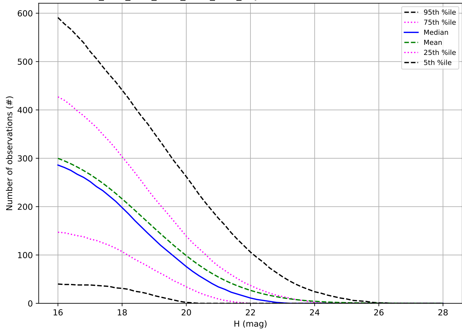
ddf_acor_sf10_lsf20_lsr50_v3.4_10yrs: Number of observations PHA
