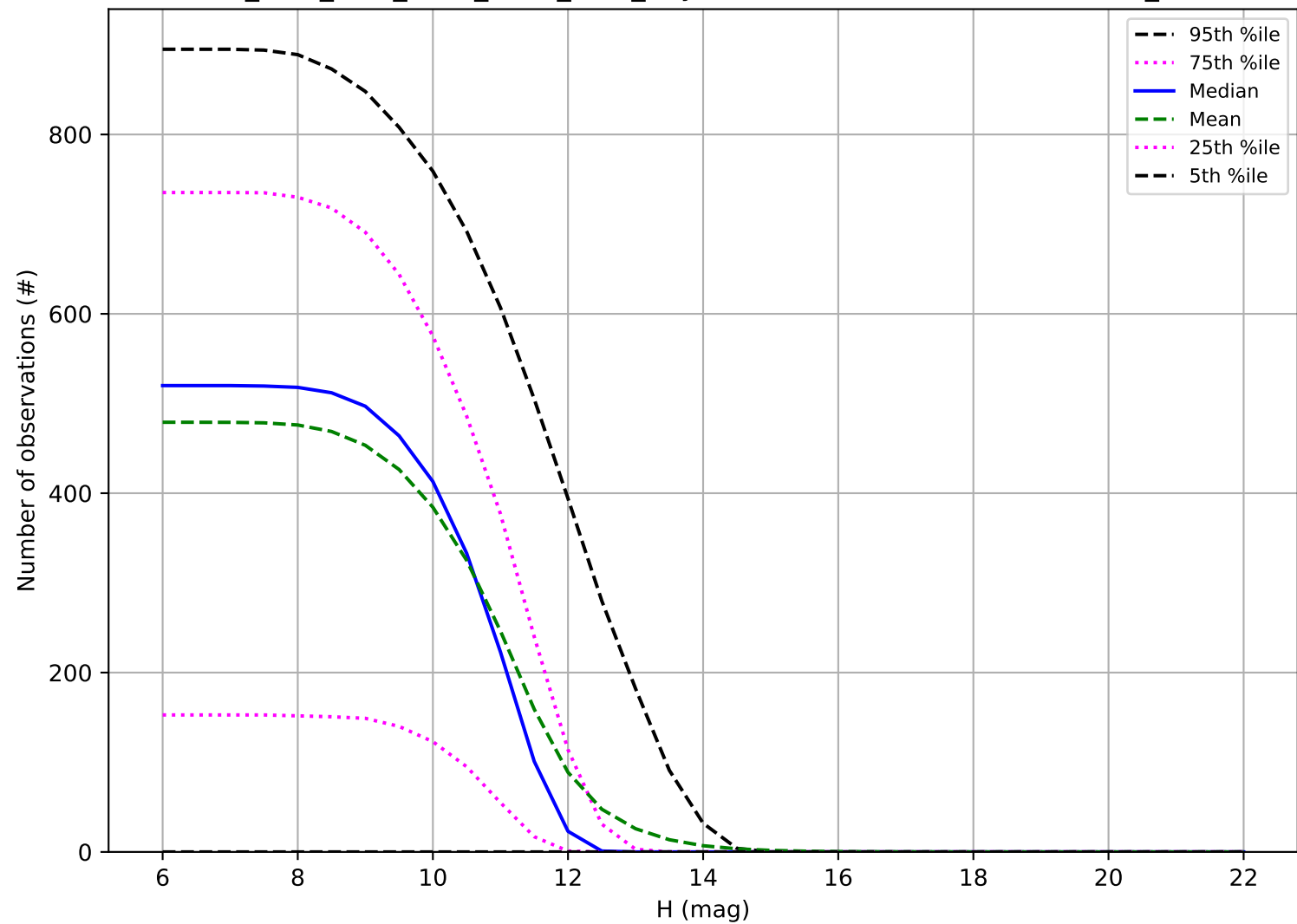
ddf_acor_sf10_lsf20_lsr50_v3.4_10yrs: Number of observations OCC_r20
