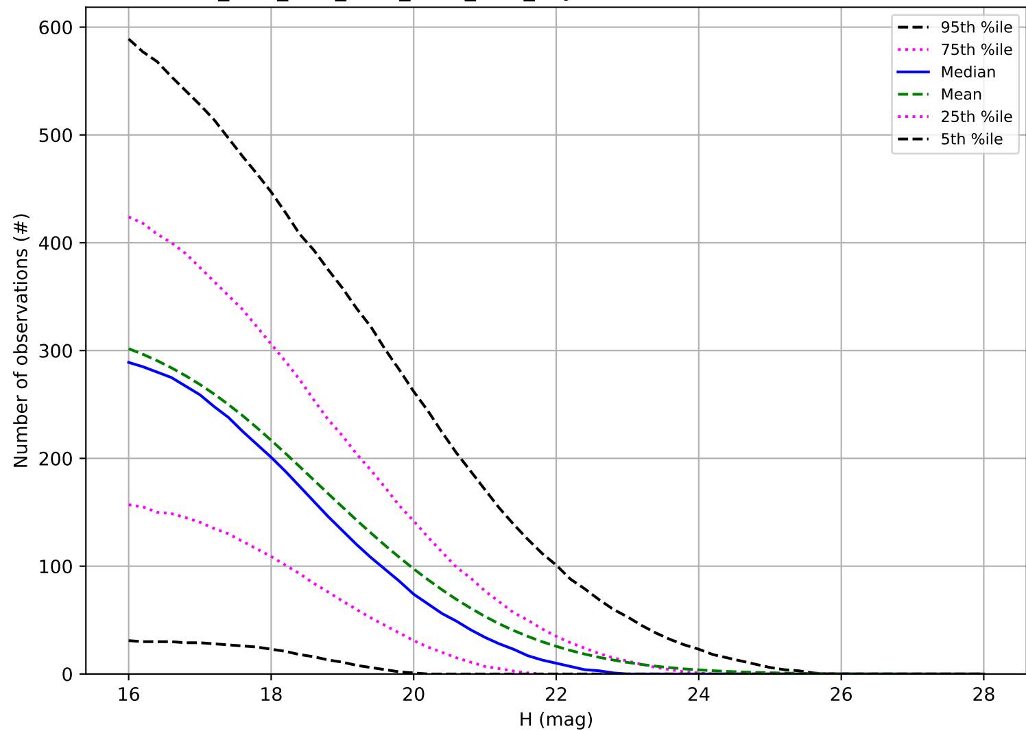
ddf_acor_sf10_lsf20_lsr50_v3.4_10yrs: Number of observations NEO
