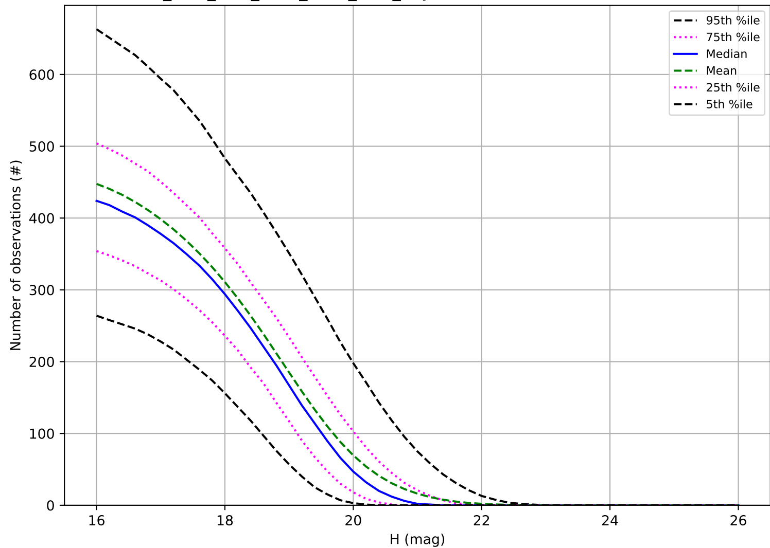
ddf_acor_sf10_lsf20_lsr50_v3.4_10yrs: Number of observations MBA
