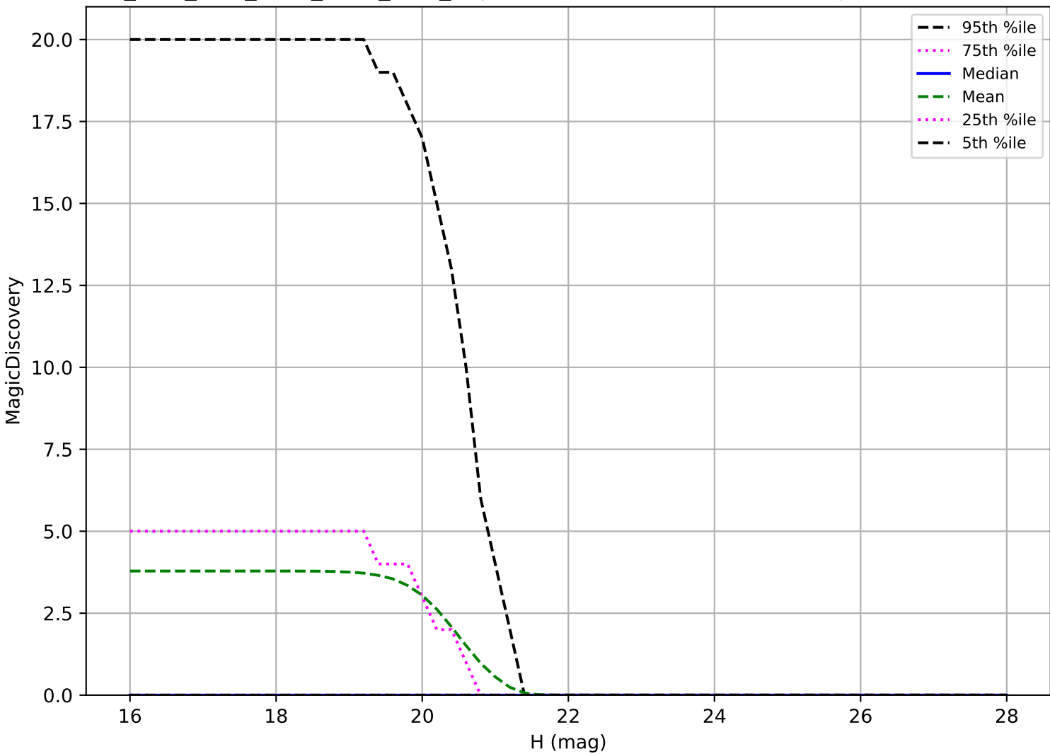
ddf_acor_sf10_lsf20_lsr50_v3.4_10yrs: Vatra 6 detections in 60 nights detection loss
