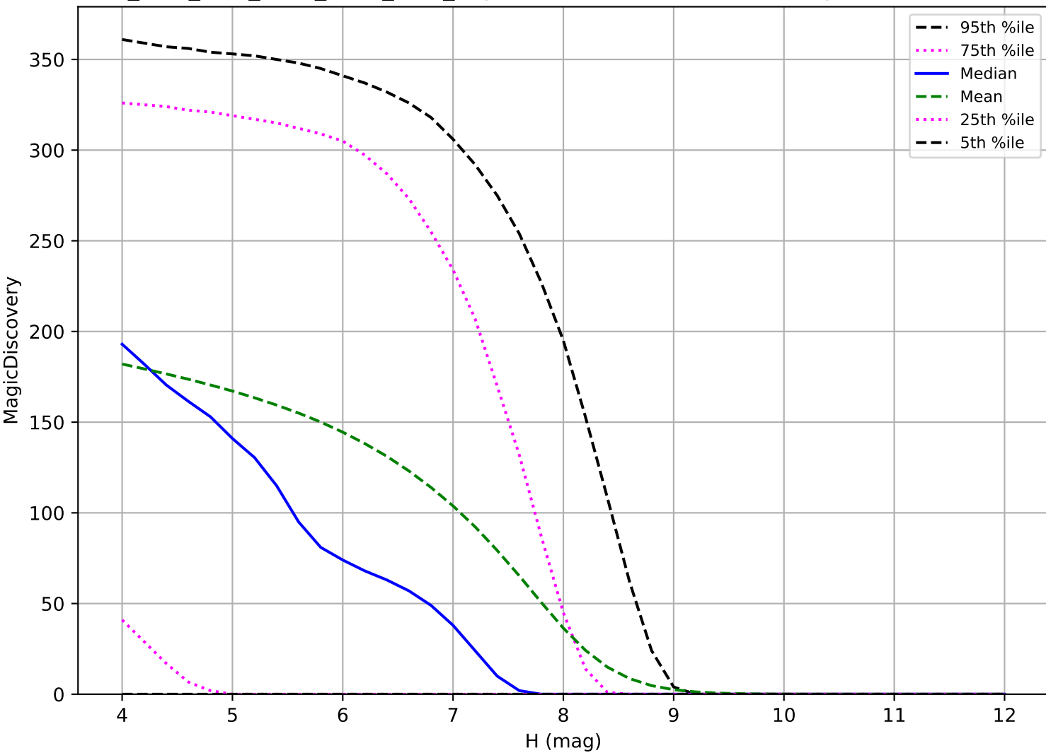
ddf_acor_sf10_lsf20_lsr50_v3.4_10yrs: TNO 6 detections in 60 nights detection loss
