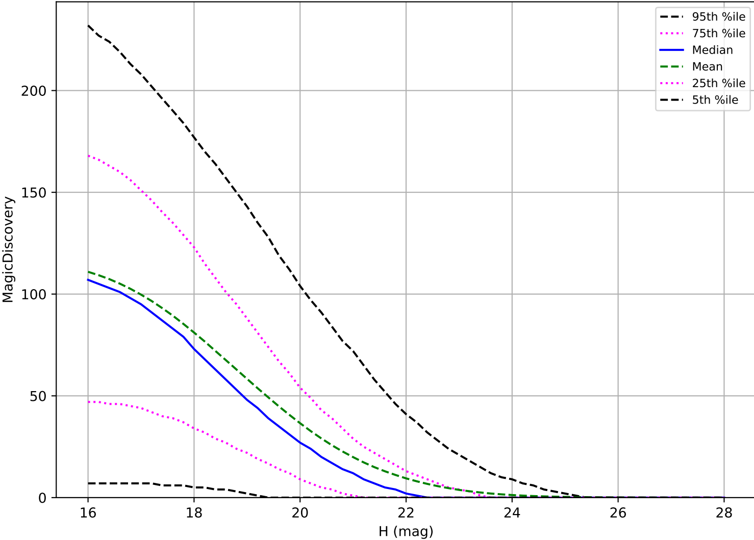
ddf_acor_sf10_lsf20_lsr50_v3.4_10yrs: PHA 6 detections in 60 nights detection loss
